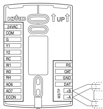
Illustration 7–1 BACnet MS/TP network wiring
