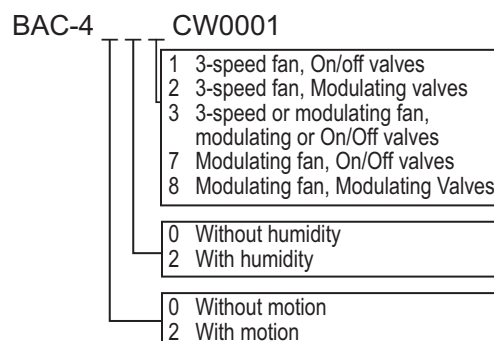
Illustration 1–1 Model numbers for fan coil units
